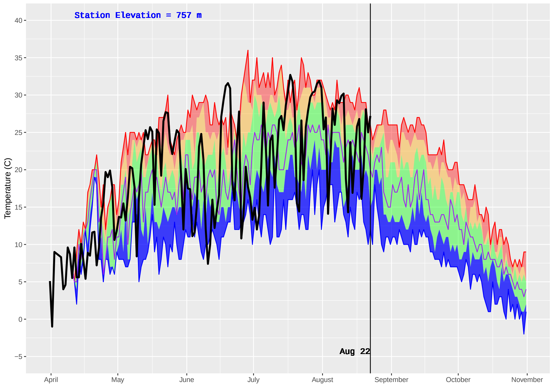
DOWNIE (905) : Historical (2005–2016) and Current (2018) Daily Temperature
